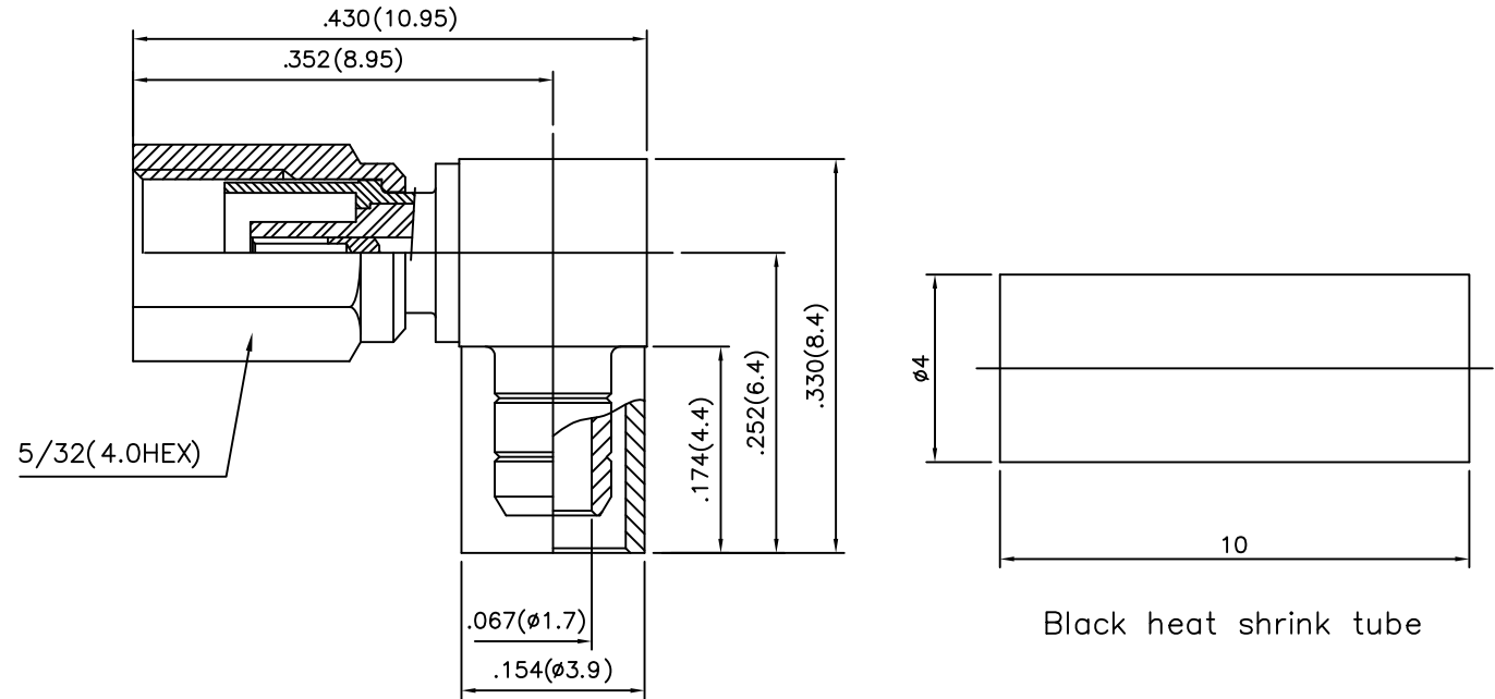
SSMC Right Angle Cable Plug for RG316 Crimp
