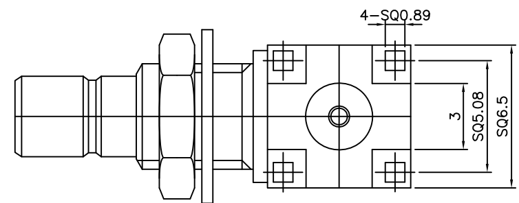
SMB-Right Angle Bulkhead Jack PCB MOUNT
