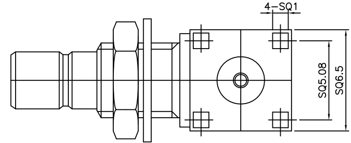
SMB-Right Angle Bulkhead Jack PCB MOUNT
